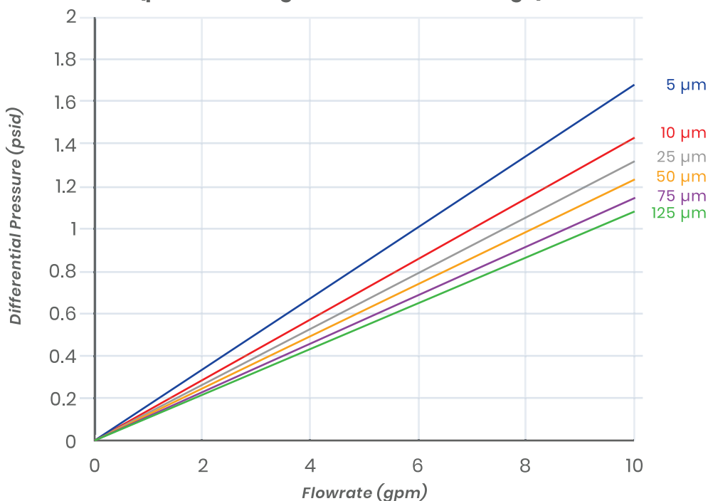
Typical Flow Rate Clean Water at Ambient Temperature (per 10" non-grooved MAB cartridge)
